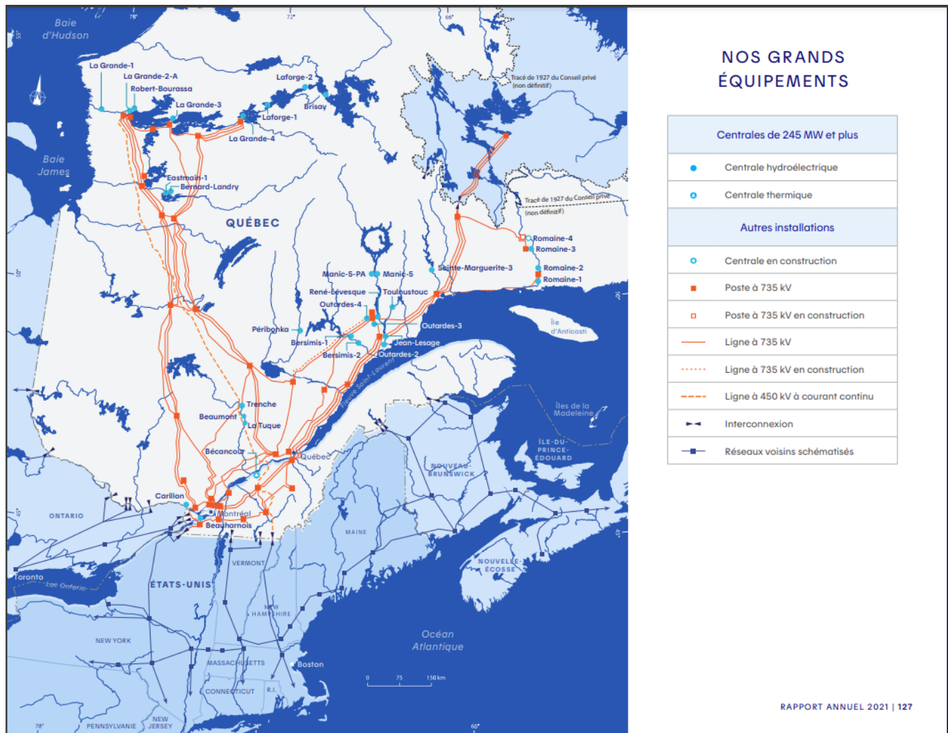
Figure 10-21: Hydro-Québec Major Infrastructure and Equipment
