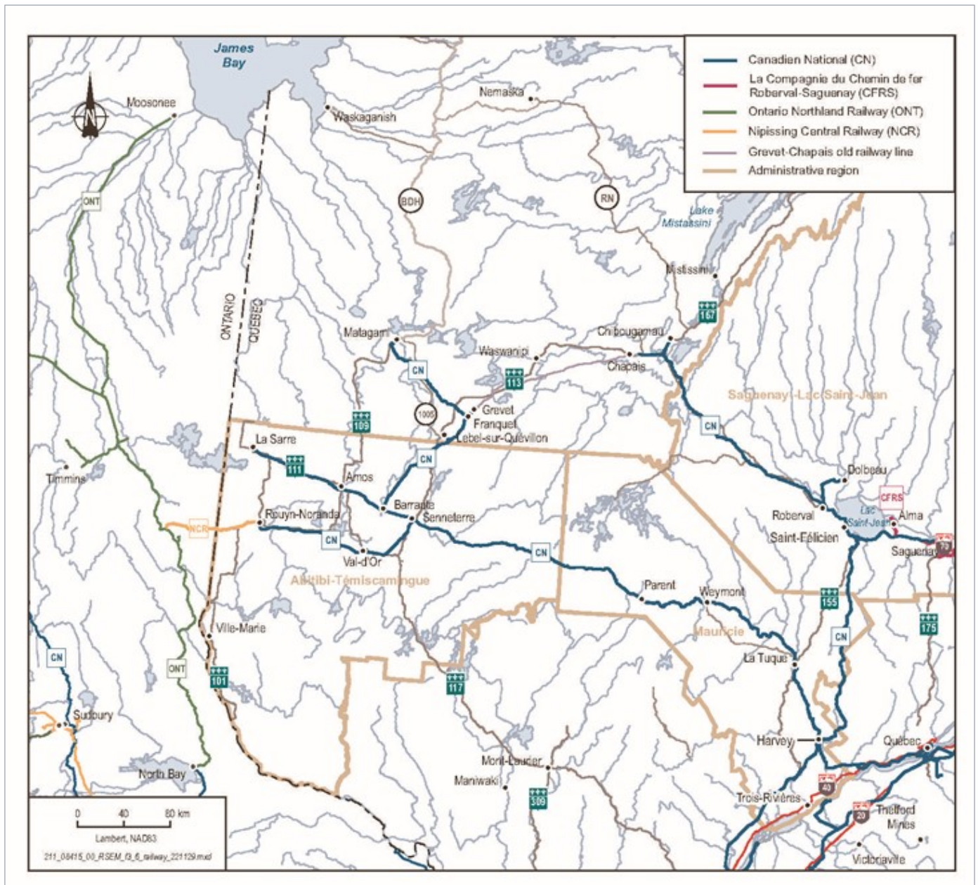
Figure 10-12: Central Northern Quebec Railway Infrastructure
